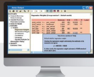
AMOS Version 24
