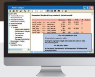
AMOS Version 24
