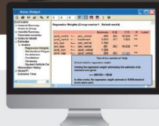
AMOS Version 24
