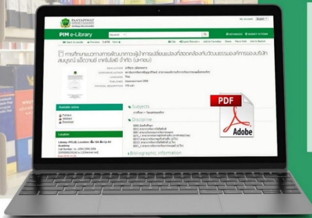
e-Collections Website
